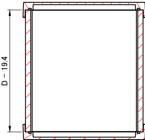
C-C (1:3)
