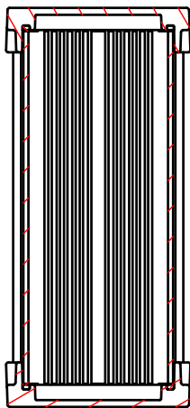
B-B (1:3)
